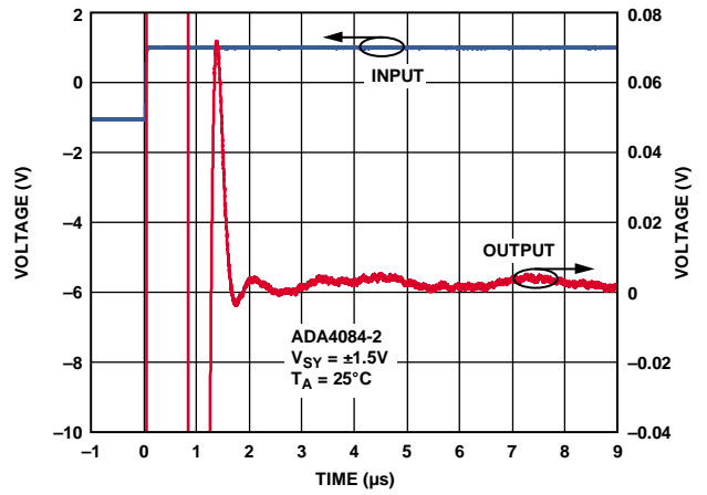
Figure 20. Settling Time
