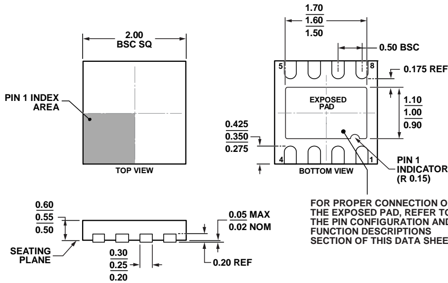
Figure 55. 8-Lead Lead Frame Chip Scale Package [LFCSP_UD] 2 mm x 2 mm Body, Ultra Thin, Dual Lead (CP-8-10)
