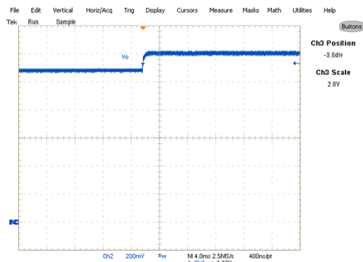
Fig. 9: Start up with 1V Pre Bias , 0A Load, Ch 2 : V_o
