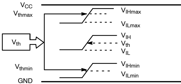
Figure 8. V_{th} Diagram
