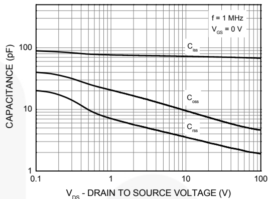
Figure 8. Capacitance
