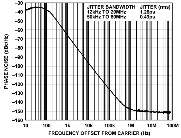
Figure 7. Phase Noise ( f_{REF} = 19.44 \text{ MHz} , f_{OUT1} = 155.52 \text{ MHz} )
