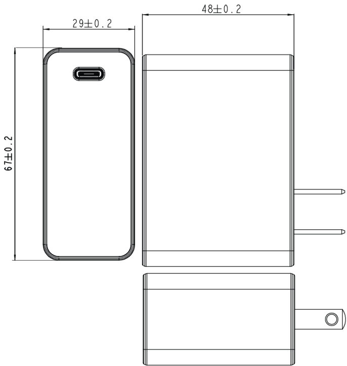
AQ36A-5CFA-H Dimension Diagram Unit: mm
