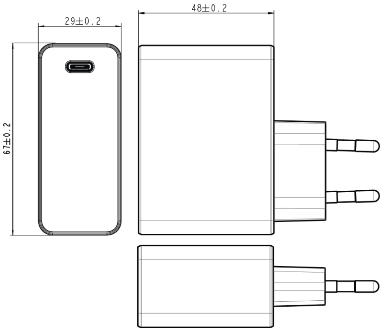
AQ36E-5CFA-H Dimension Diagram Unit: mm
