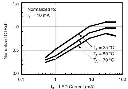
Figure 6. Normalized CTR_{cb}
