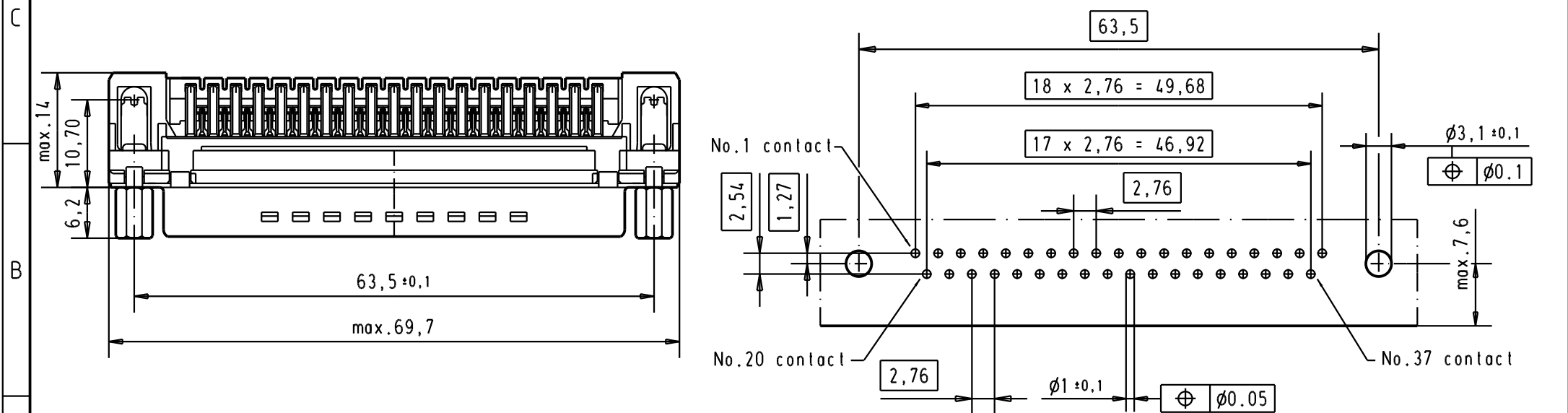
Printed board layout component side
