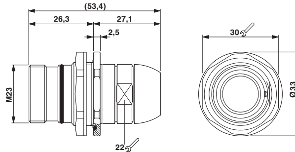
Dimensional drawing
