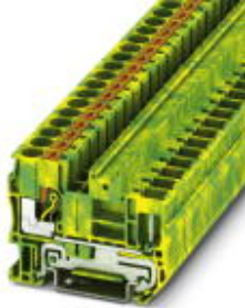
Feed-through terminal block, Connection method: Push-in / plug connection, Cross section: 0.5 mm² - 10 mm², AWG: 20 - 8, Width: 8.2 mm, Color: green-yellow
