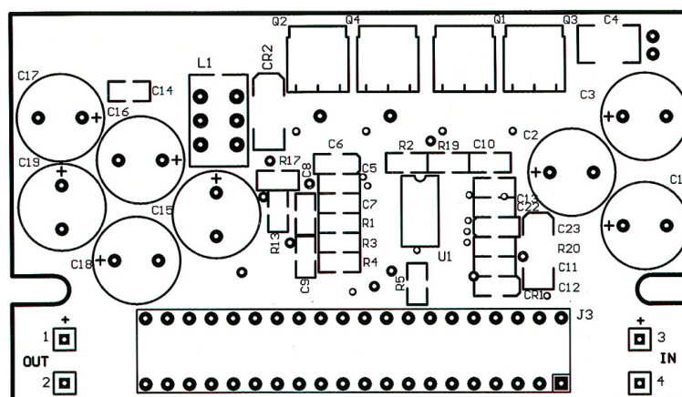
FIGURE 2. Si9143DB Top Layer Silk Screen
