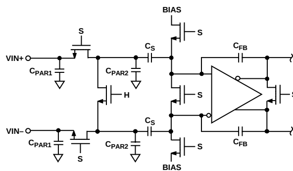
Figure 35. Switched Capacitor Input
