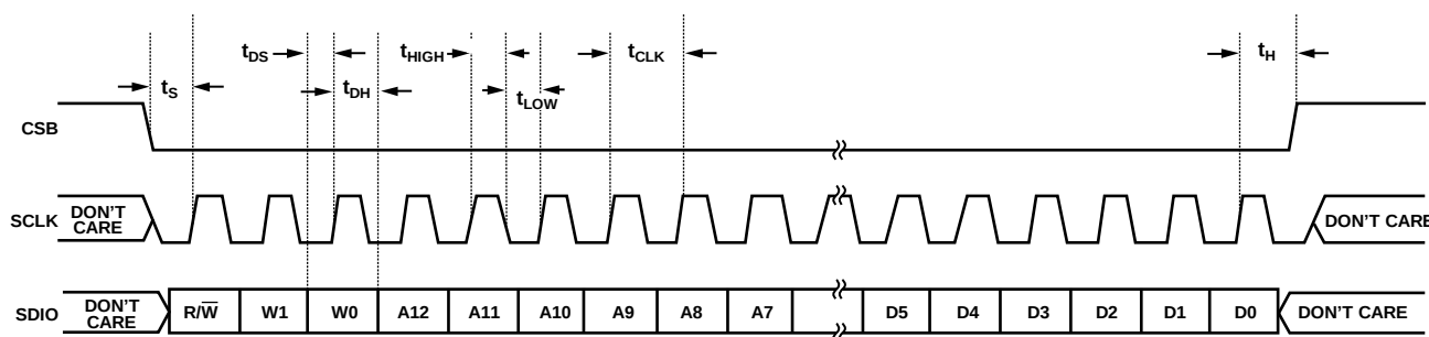
Figure 60. Serial Port Interface Timing Diagram
