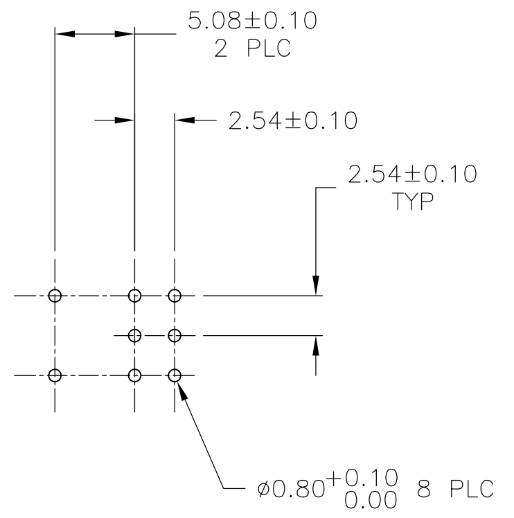
RECOMENDED P.C. HOLE LAYOUT DOUBLE POLE
