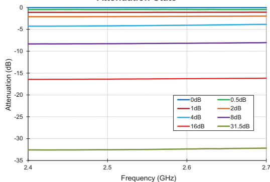
Normalized Attenuation versus Attenuation State
