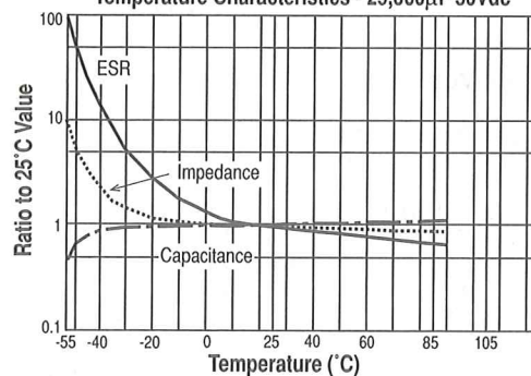
Temperature Characteristics - 29,000 \mu F 50Vdc
