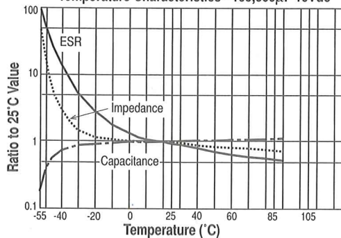
Temperature Characteristics - 100,000 \mu F 10Vdc
