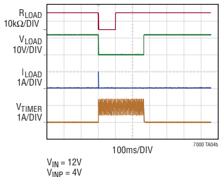
R_{TIMER} = OPEN 12 \Omega /100ms LOAD PULSE
