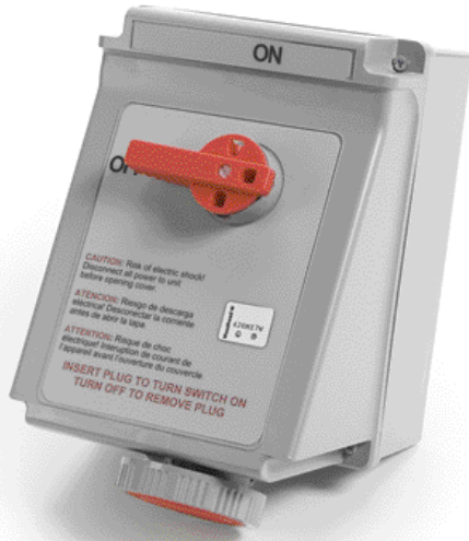
MECHANICAL INTERLOCK
