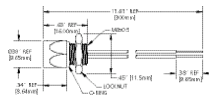
FEMALE RECEPTACLE (ACCOMMODATES THREADED MALE CORDSETS ONLY)
