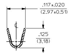
SECT. "B-B"
