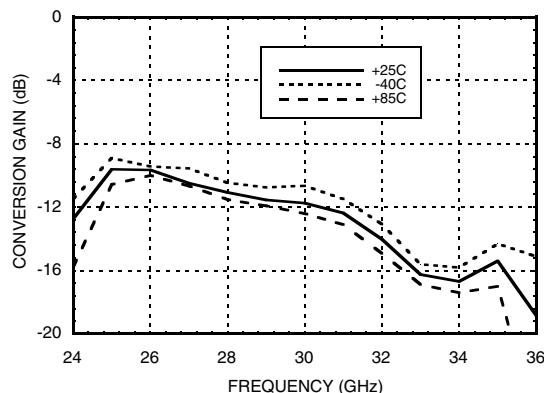
Conversion Gain vs. Temperature @ LO = -4 dBm, Vdd = +4V
