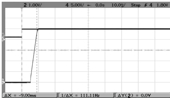
On/Off Enable Delay (Vin=13.8V, Vout=5V, Iout=6.1A, Cload=0) Trace 4=Enable, Trace 2=Vout
