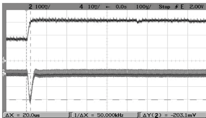
Step Load Transient Response (Vin=12V, Vout=5V, Cload=0, Iout=3A to 6A) Trace 2=Vout, 100 mV/div. Trace 4=Iout, 2A/div.
