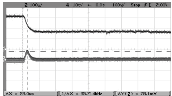
Step Load Transient Response (Vin=12V, Vout=2.5V, Cload=0, Iout=6A to 3A) Trace 2=Vout, 100 mV/div. Trace 4=Iout, 2A/div.
