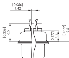
52 Contact design Kontaktvariante Line Contact Termination Kontaktlamellenanschluss
