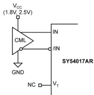
Figure 4a. CML Interface (DC-Coupled, 1.8V, 2.5V)
