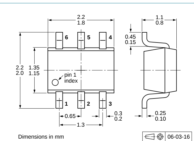
Fig 17. Package outline PUMD18 (SOT363)
