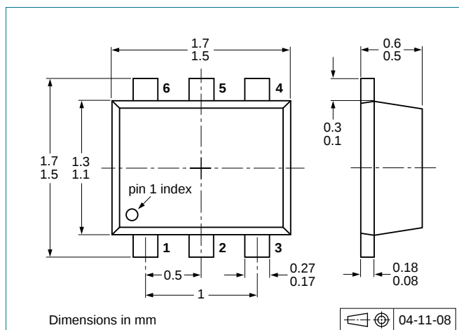
Fig 16. Package outline PEMD18 (SOT666)
