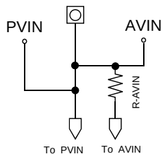
Solder Land_PVIN
