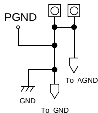
Solder Land_GND
