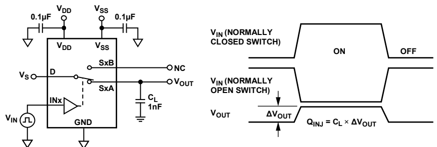
Figure 30. Charge Injection
