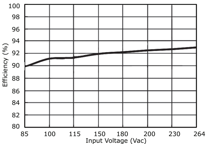
PDRA-120-24 Efficiency Curve (Efficiency vs. Input Voltage)
