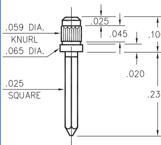
1216-0-05-XX-00-00-01-0 Press-fit in .056 mounting hole
