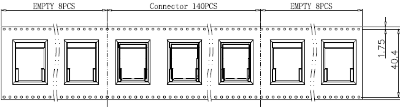
DIMENSIONS: mm
