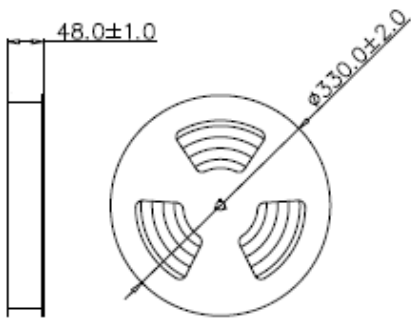
DIMENSIONS: mm
