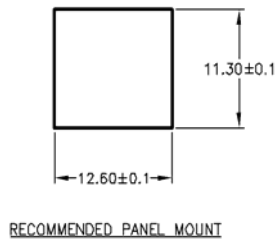
RECOMMENDED PANEL MOUNT
