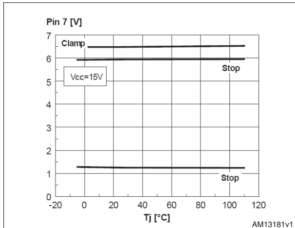
Figure 19. Latched disable threshold vs. junction temperature
