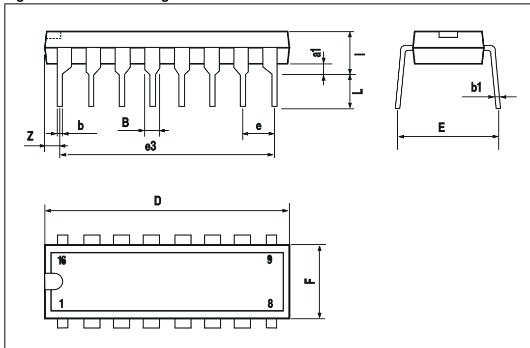
Figure 33. DIP16 drawing
