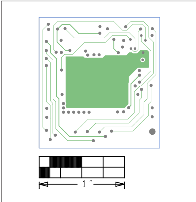
MAX86140OSBEK#—L03_SIG
