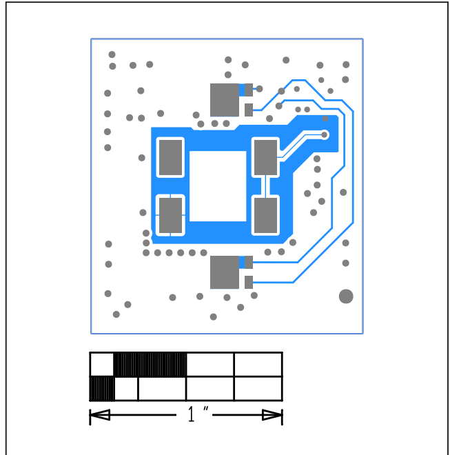
MAX86140OSBEK#—BOTTOM
