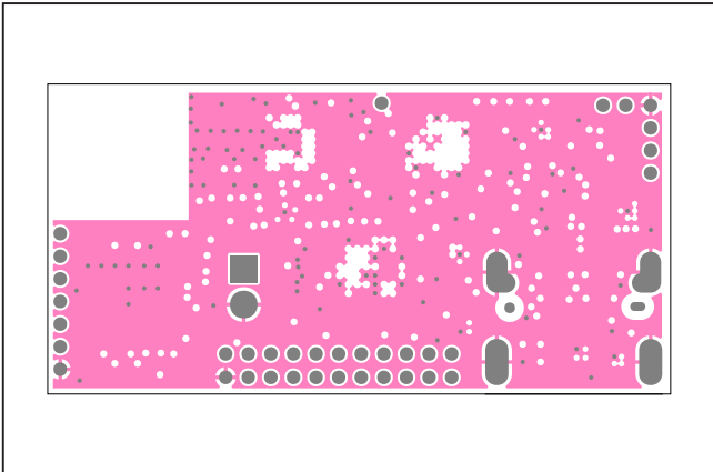
MAXSensorBLE_EVKIT—L11_GND
