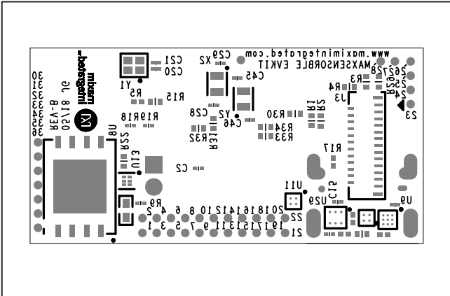
MAXSensorBLE_EVKIT—SILK_BOT
