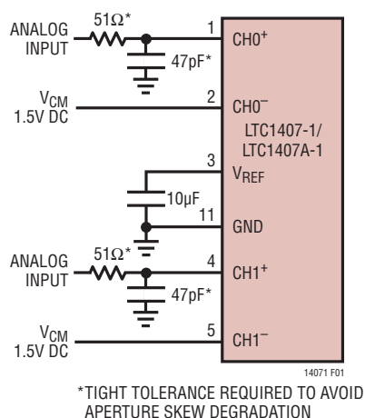
Figure 1. RC Input Filter
