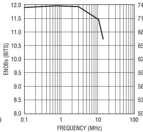
ENOBs and SINAD vs Input Sinewave Frequency for Differential Input Signals
