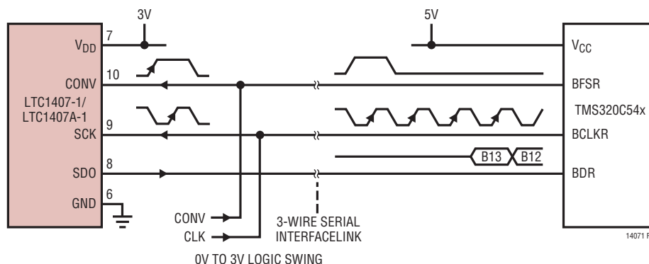
Figure 8. DSP Serial Interface to TMS320C54x
