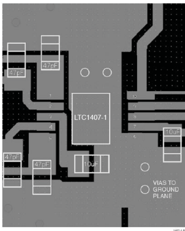
Figure 7. Recommended Layout
