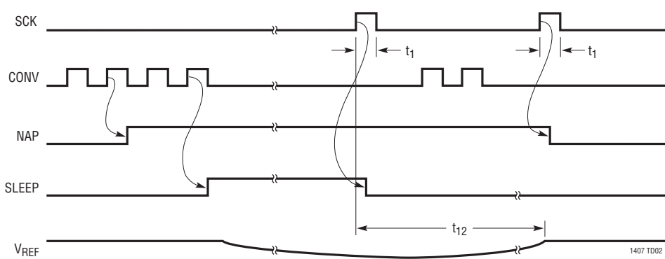
Sleep Mode Waveforms
