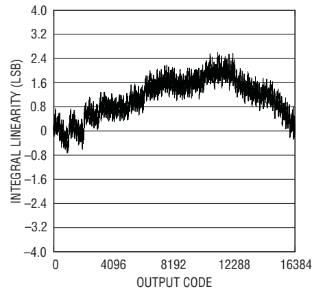
Integral Linearity End Point Fit for CH1 with Internal 2.5V Reference
