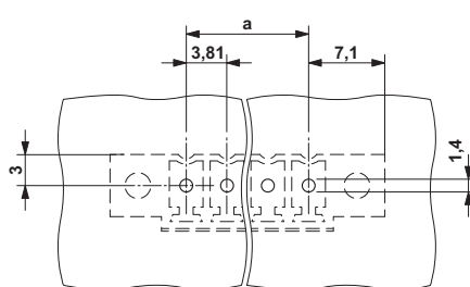
Drilling diagram
