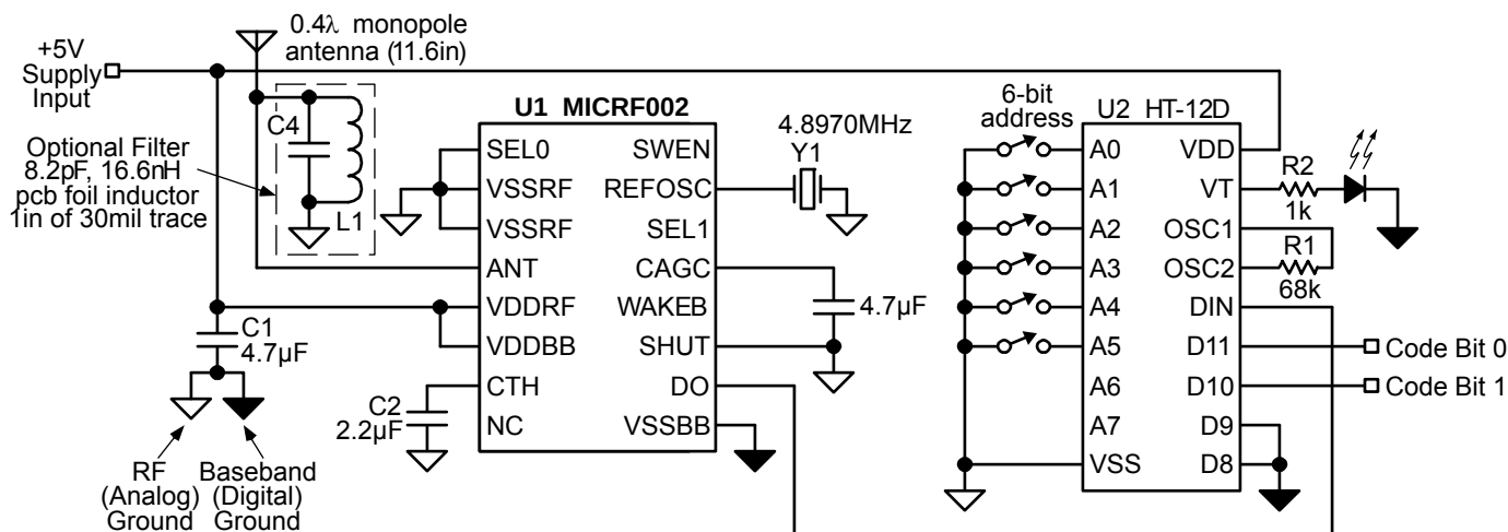
Figure 7. 315MHz, 1kbps On-Off Keyed Recwiver/Decoder
