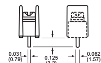
14 Printed Circuit
