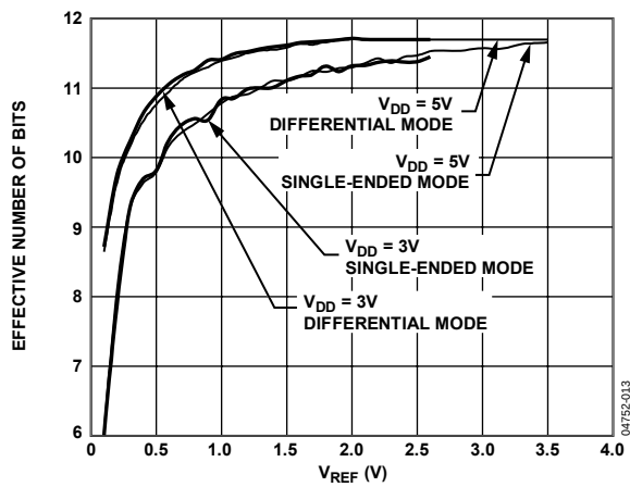
Figure 10. ENOB vs. V_{REF}
