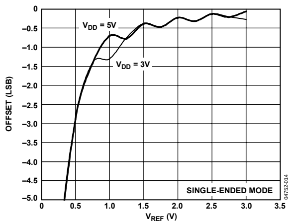
Figure 11. Offset vs. V_{REF}
