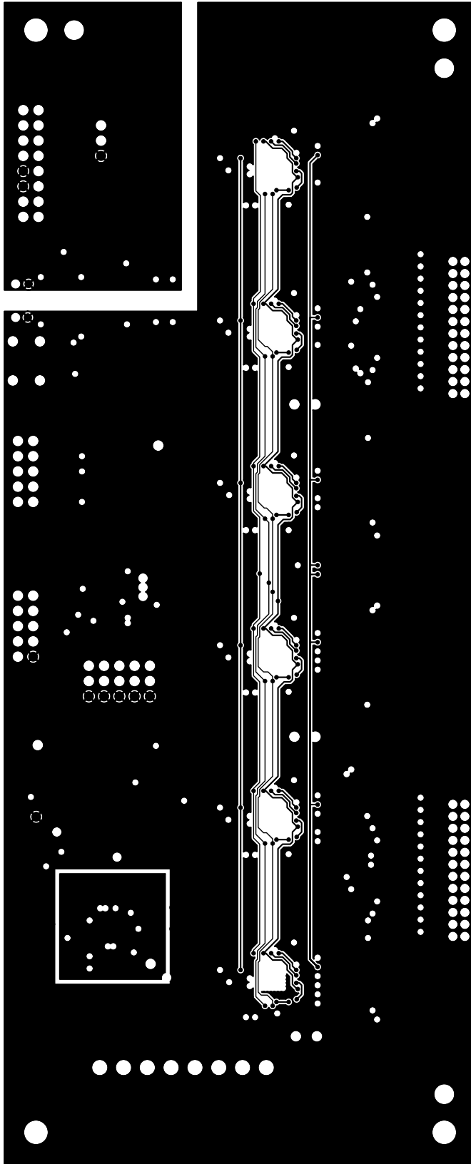
Figure 18. Smart PSE 24 Power Plane
