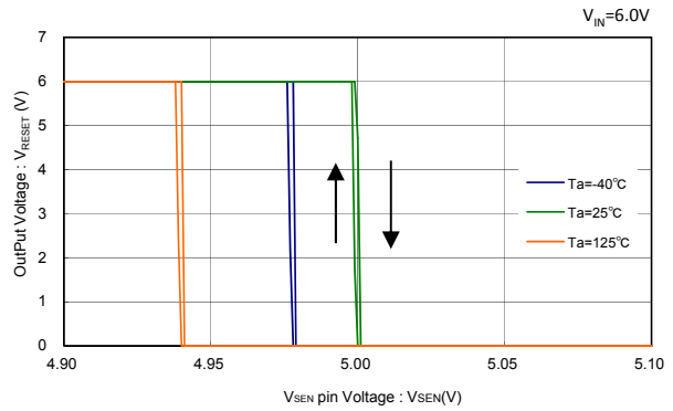
XC6134x50A ( V_{DF(T)}=5.0V )
