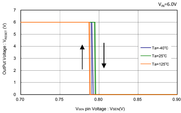
XC6134x08A ( V_{DF(T)}=0.8V )
