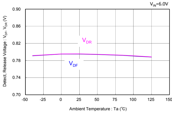
XC6134 ( V_{DF(T)}=0.8V )
