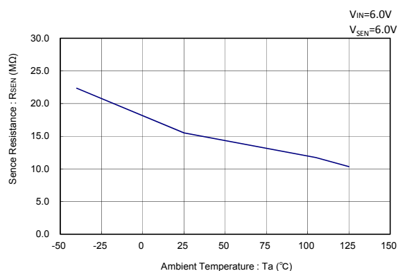
XC6134 ( V_{DF(T)}=0.8V )
