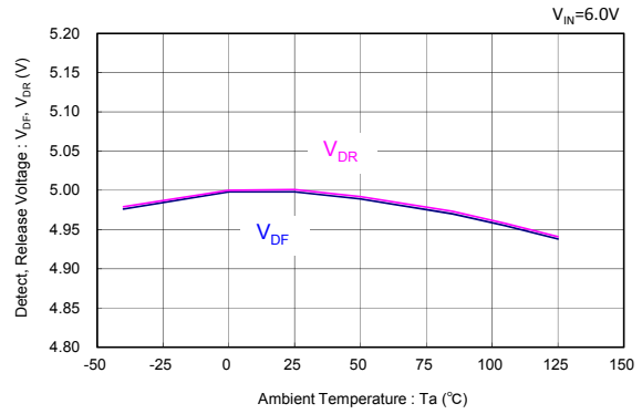
XC6134 ( V_{DF(T)}=5.0V )
