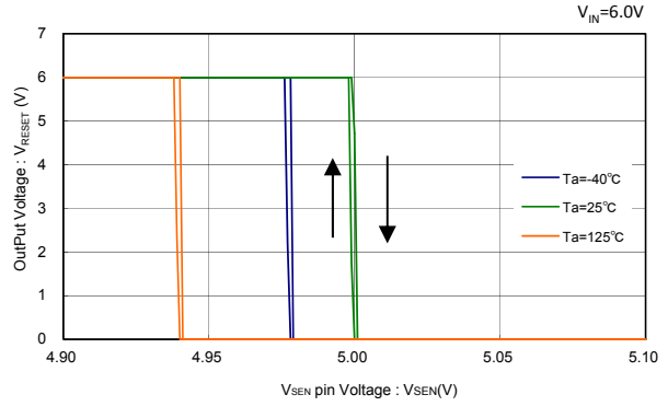
XC6134x50A ( V_{DF(T)}=5.0V )
