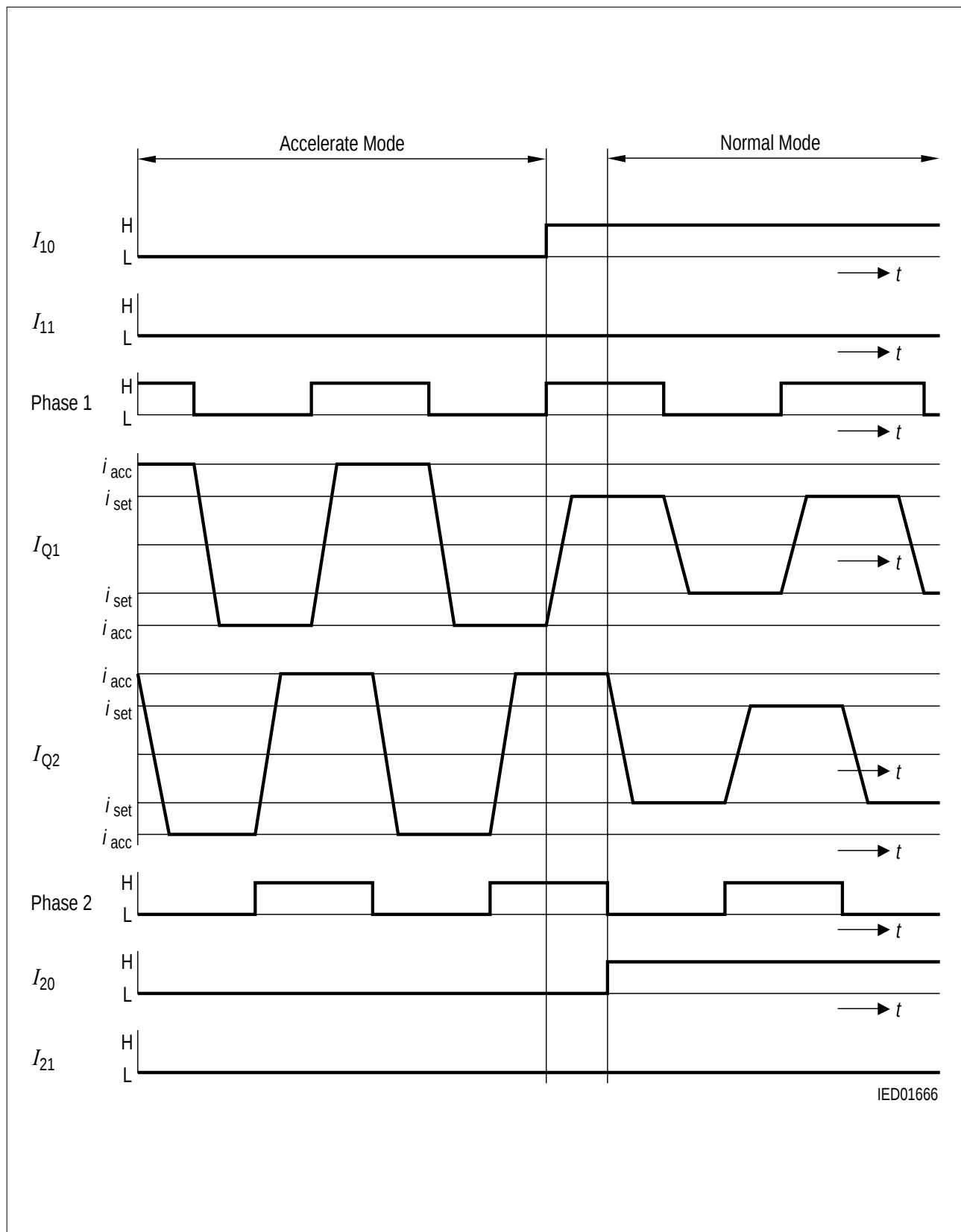
Figure 5 Full-Step Operation
