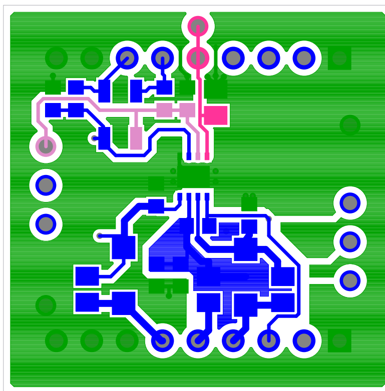
FIGURE 10. TOP LAYER
