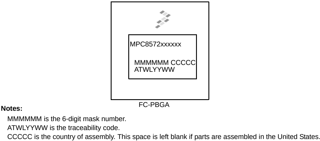
Figure 67. Part Marking for FC-PBGA Device
