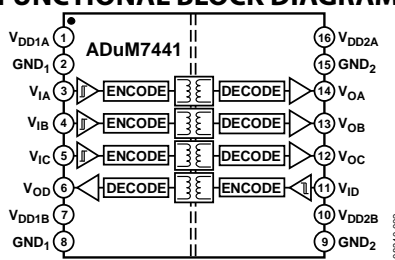
Figure 2. ADuM7441
