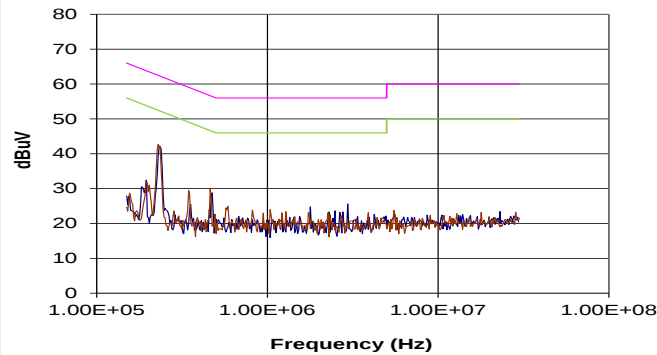
CRE1S0505MC
