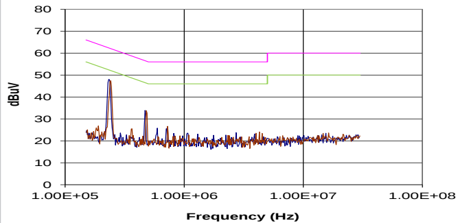
CRE1S1212SC
