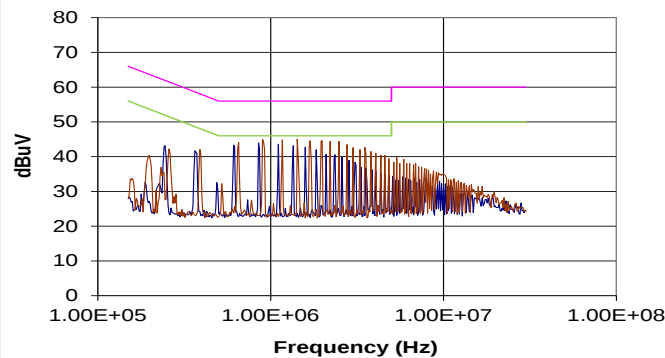
CRE1S0505MC
