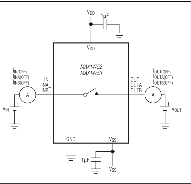
Figure 3. Off-Leakage Current
