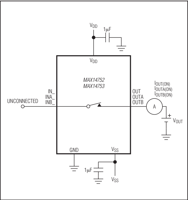
Figure 2. On-Leakage Current
