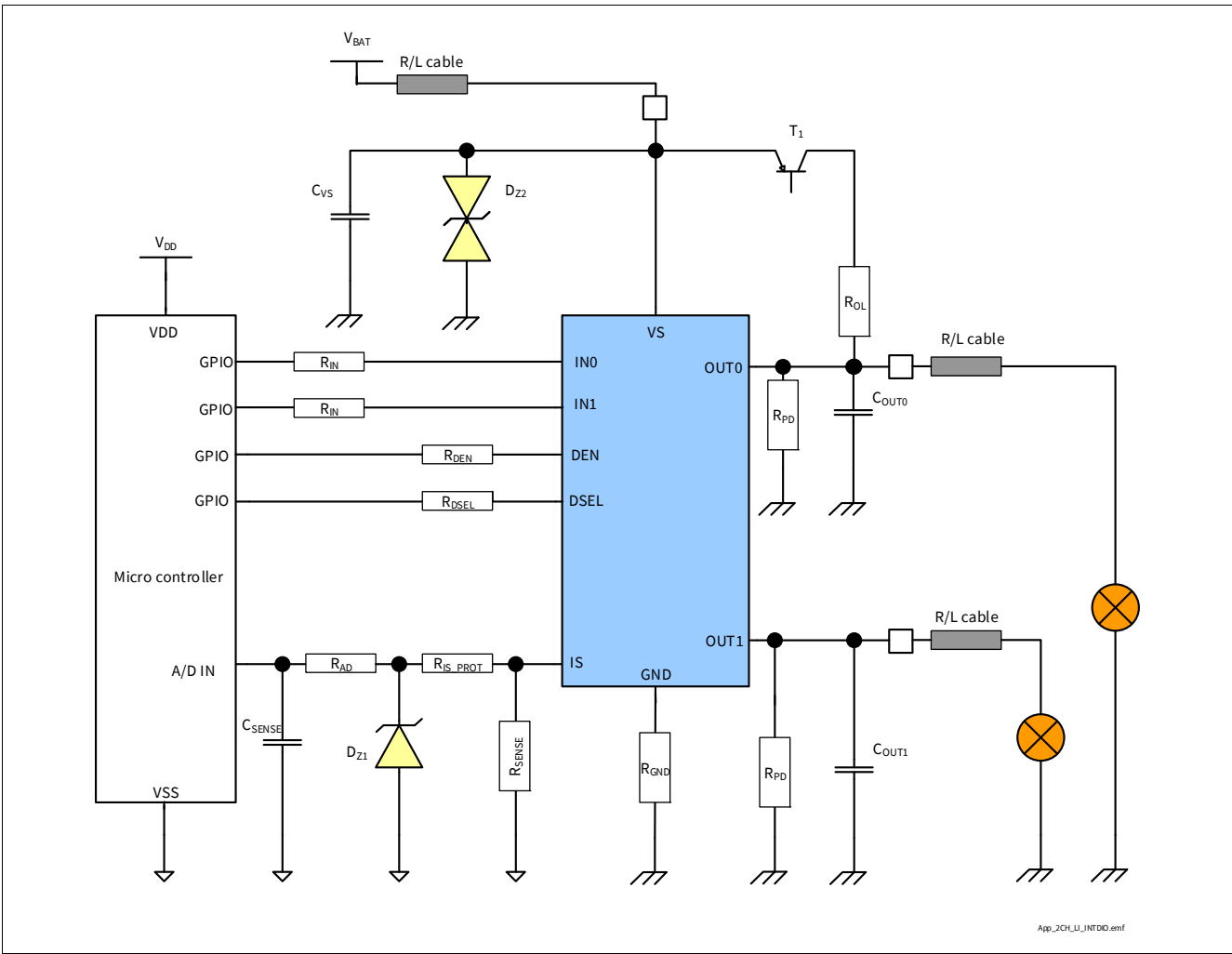
Figure 42 BTS7120-2EPA Application Diagram
