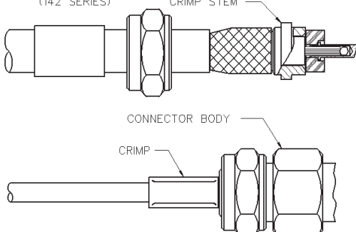
RG-58, RG-142 CABLE GROUP (142 SERIES)
