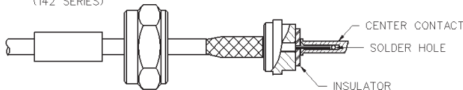
RG-58, RG-142 CABLE GROUP (142 SERIES)
